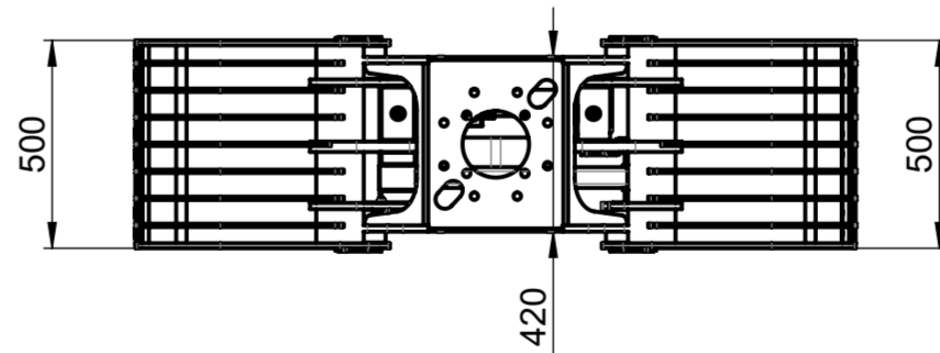
BEHA BUG-A 7-9 305 kg
