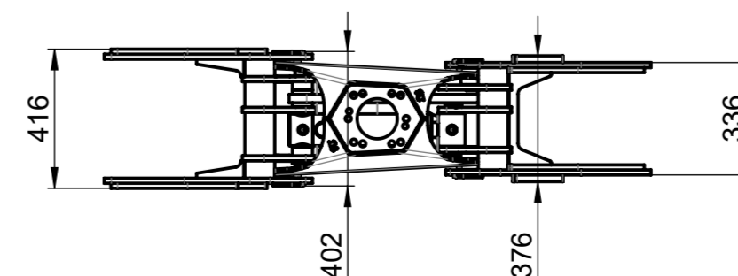
BG026/R4 Reissiggreifer 160 kg
