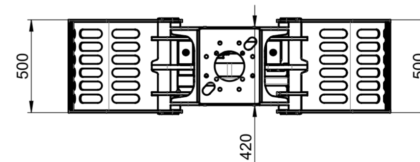
BEHA BUG-W 7-9 285.38 kg
