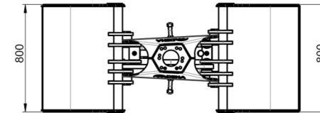
BKG 400 Krangreifer 370 kg
