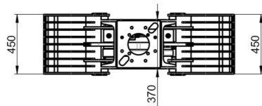
BEHA BUG-A 5-7 235 kg
