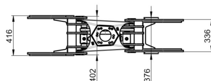
BG026/R4 Reissiggreifer 160 kg
