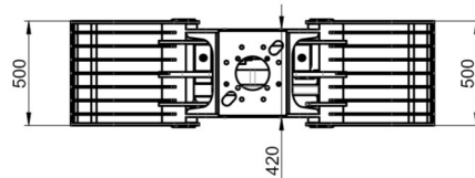
BEHA BUG-A 7-9 305 kg
