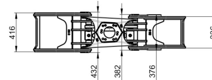
BG026/S Holzgreifer 200 kg
