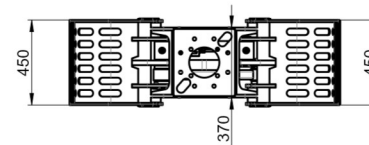
BEHA BUG-W 7-9 285.38 kg
